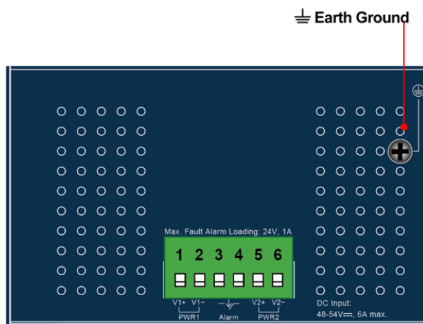
Figure 3-5: Grounding Method (applies to all models)
