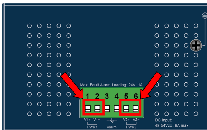
Figure 3-1: IGS-4215-4P4T/IGS-4215-4P4T2S/IGS-4215-8P2T2S DC Inlet Power Socket
