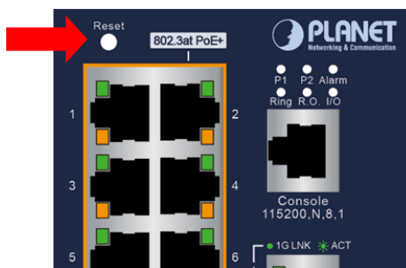
Figure 6-2: IGS-4215-16P2T2S Reset Button
