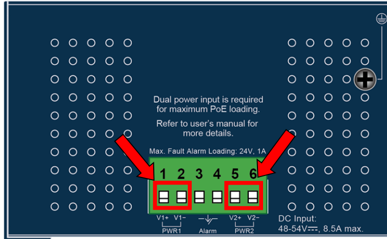
Figure 3-2: IGS-4215-4UP4T2S/IGS-4215-8UP2T2S DC Inlet Power Socket
