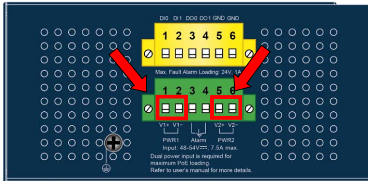
Figure 3-3: IGS-4215-16P2T2S DC Inlet Power Socket
